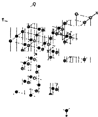
FIG. 64.—Triclinic Space-Lattice.
